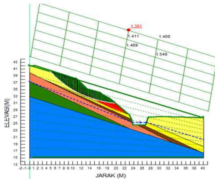
Figure 3. Slope Stability Analysis of the Bishop Method Using Geostudio2018 Software
