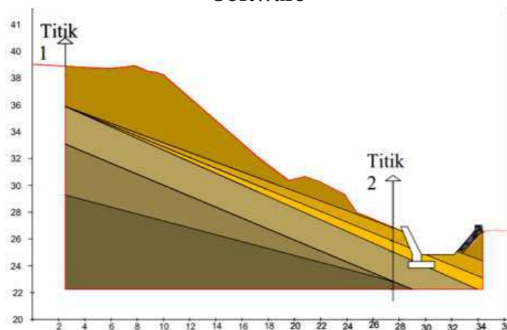
Figure 4. Retaining Wall Placement Plan
