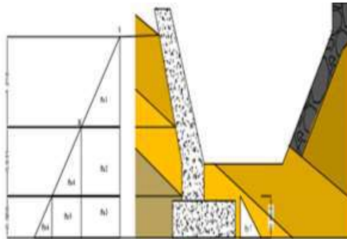
Figure 5. Active and Passive Soil Diagrams
