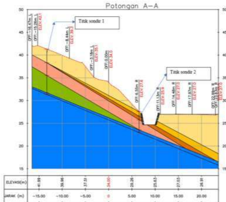
Figure 2. Topographic Data in the form of Cross Sections
