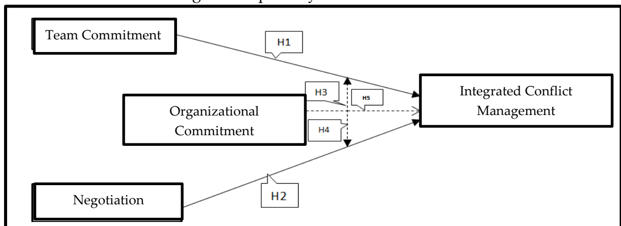
Figure 1. Research Model
